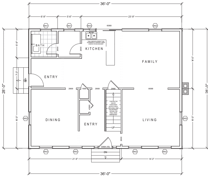
FIRST FLOOR
